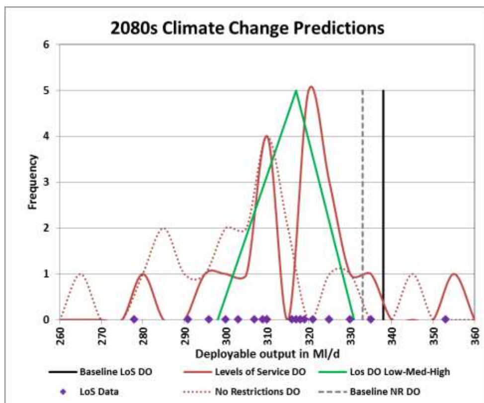
Figure 10: 2080s climate change predictions
