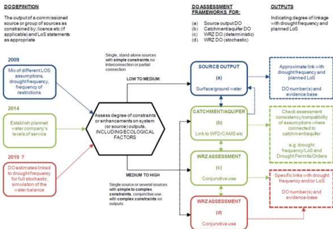
Figure 7: Deployable output analysis
