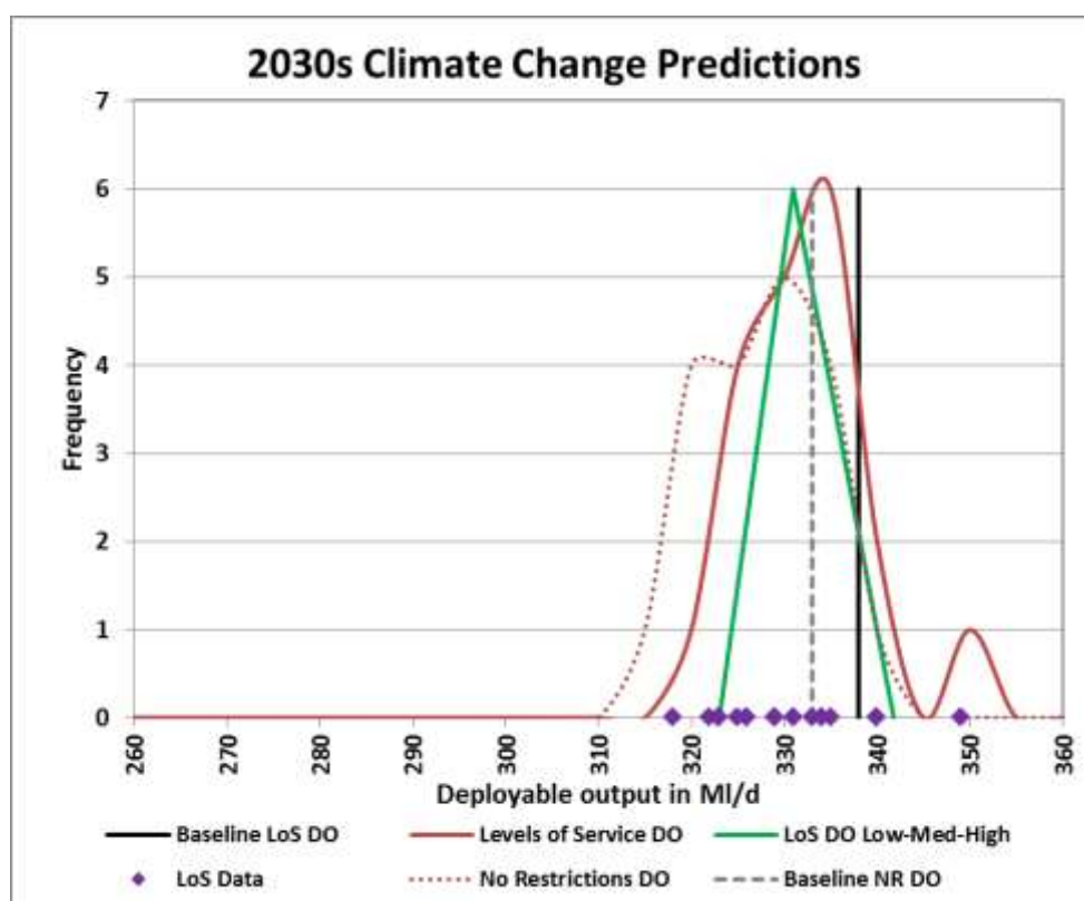
Figure 11: 2030s climate change predictions
