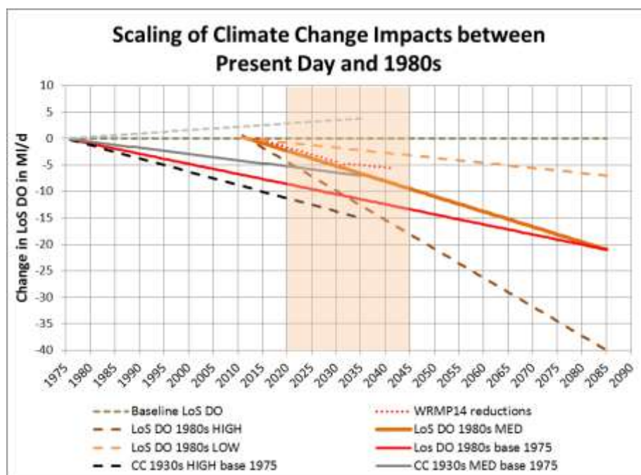
Figure 12: Scaling of climate change impacts between present day and 1980s
