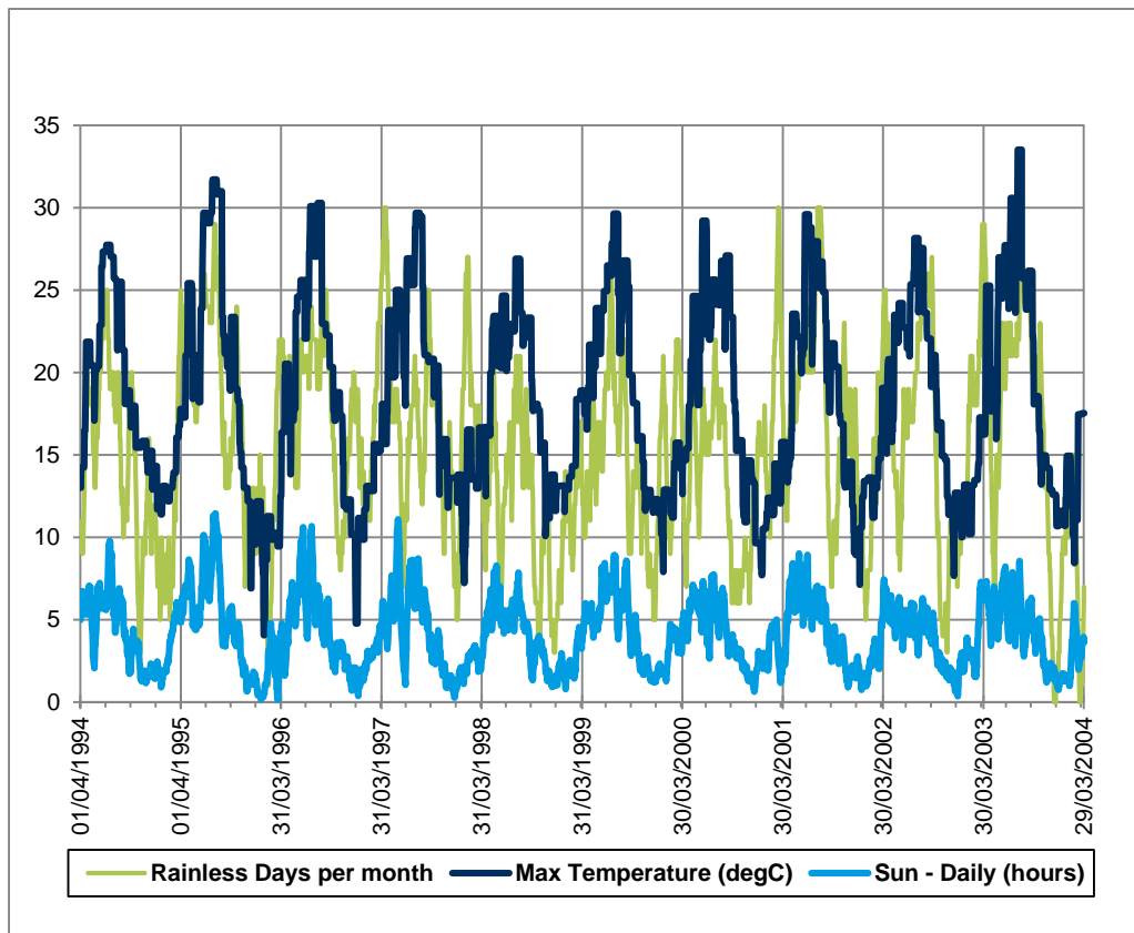
Figure 5: Temperature, sunshine hours and rainless days 1994/2004
